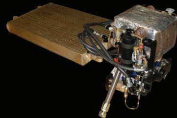
FCS Vapor Compression System Unit
